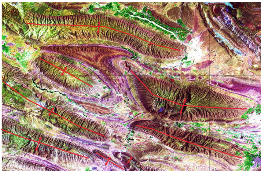
Fig. 4.8 Landsat image in false colour that shows doubly plunging anticlines in south of Iran (color figure online)
