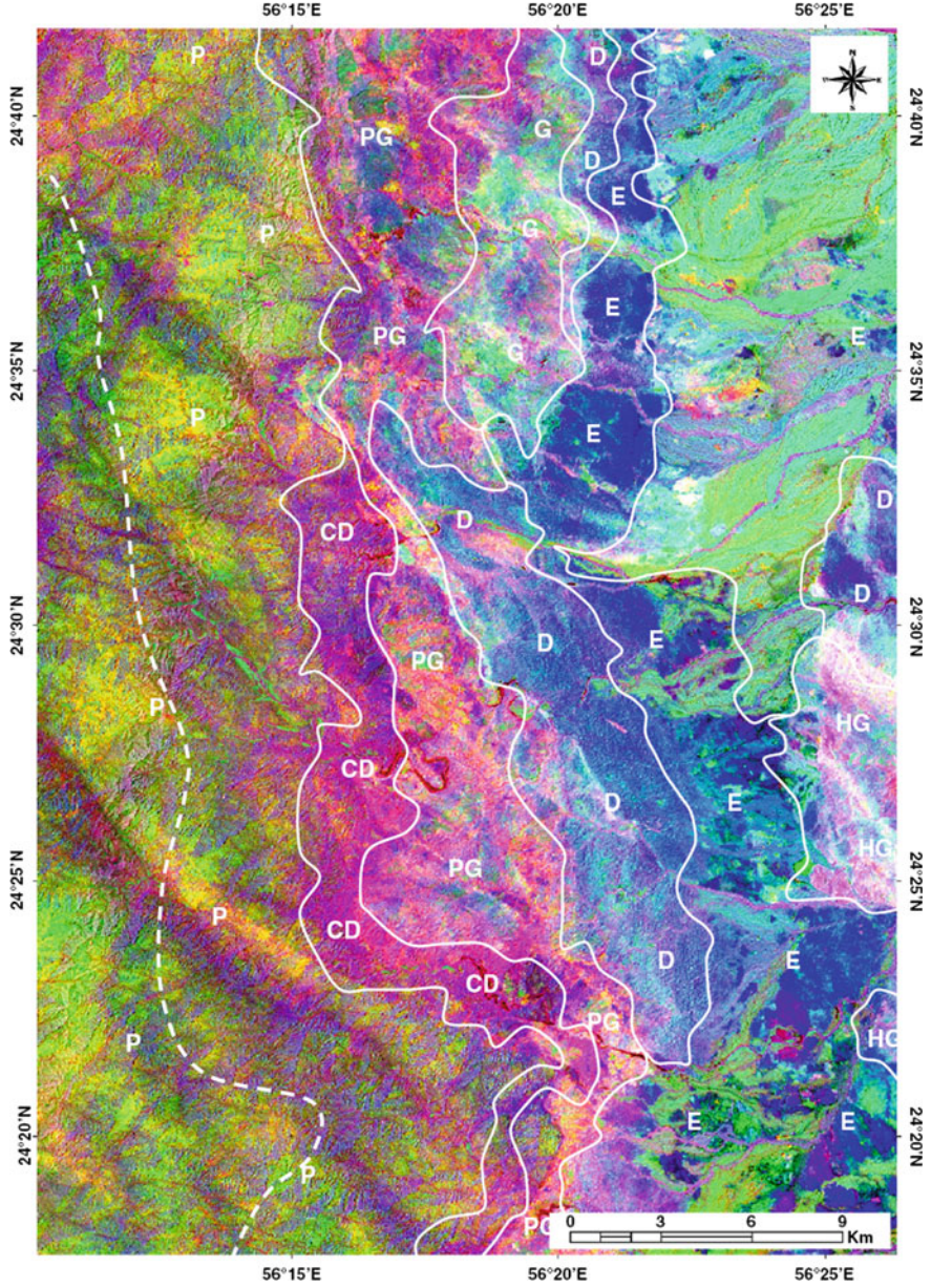
Fig. 4.24 Remote sensing image showing geology of the area; PC7, PC5 and PC4 of PCA bands. The index shows: E Basic extrusive rocks primarily spilites pillow lava, conglomerate; D Diabase dyke swarms; G Gabbro; HG Gabbroid hypabyssal rocks; PG Cumulate layered gabbro; P and CD Sheared serpentized harzburgite (adopted from Rajendran et al. 2012)
