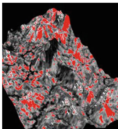
Fig. 4.20 a Carbonate fraction image and b density sliced fraction image; red <50%; green 50–60%; blue 60–70%; yellow 70–80%; cyan 80–90%; white >90% (Sanjeevi 2008) (color figure online)
