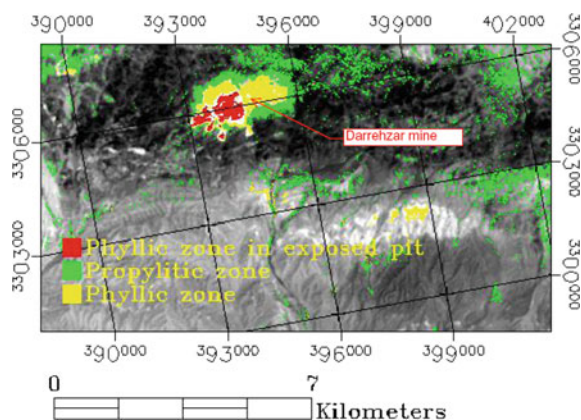
Fig. 4.18 Classified ASTER SWIR images using SAM. The map coordinate is N, UTM, Zone 40, WGS84
