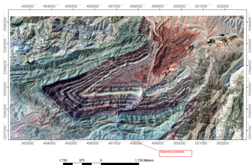
Fig. 4.7 Satellite image in true colour that shows a plunging syncline in east of Iran. The map coordinate is N, UTM, Zone 40, WGS84
