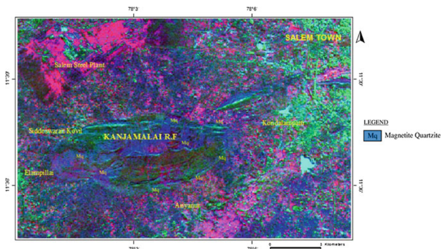
Fig. 4.23 Colour combination of band ratios ((1 + 3)/2, (3 + 5)/4, (5 + 7)/6) in red, green and blue (color figure online)
