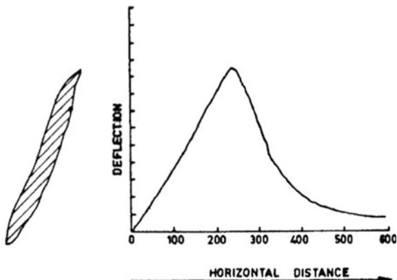
Fig. 3.1 Sulphide ore body and gravity anomaly curve
